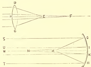
Spherical Aberration.
